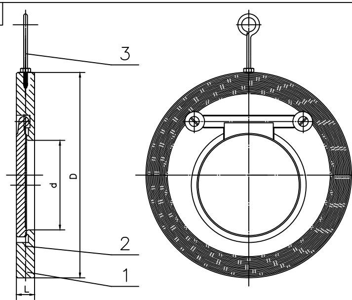
Main Dimension and Connection Size
